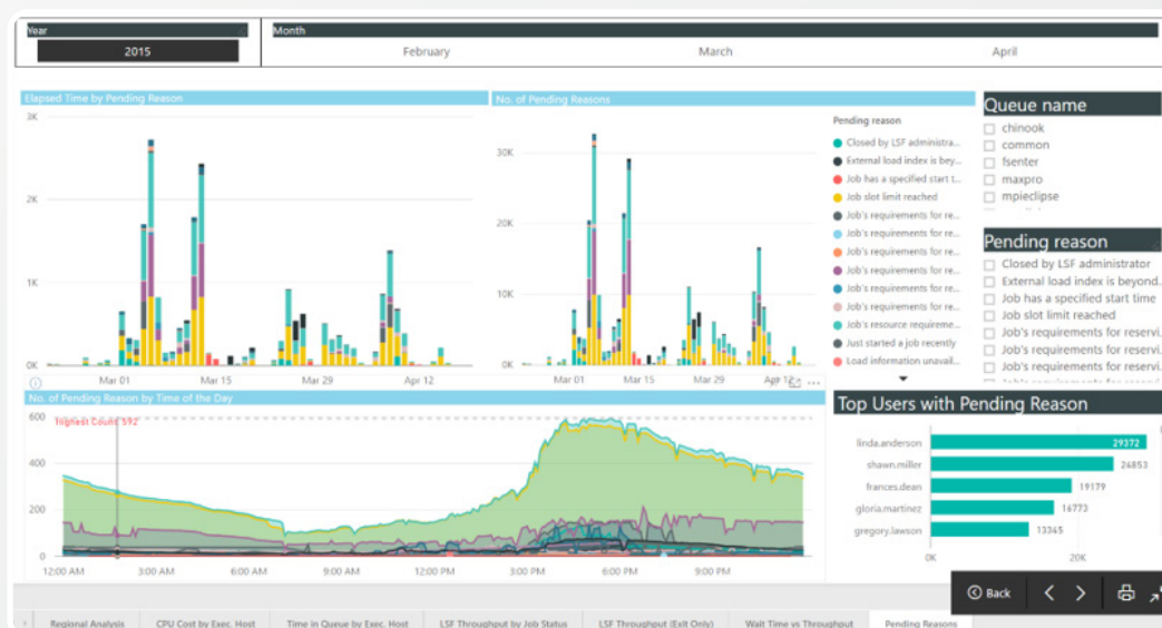
Figure 1. Dashboard do ComputeAnalyzer no Power BI
